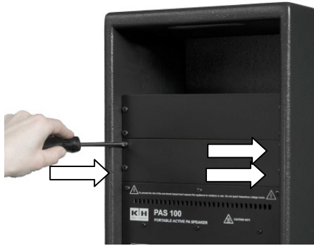
A- Unscrew the Blank Panel
