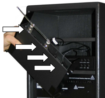
D- Attach the Audio, Power and Two Antenna Connections
